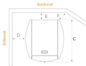
WALL CLEARANCES
